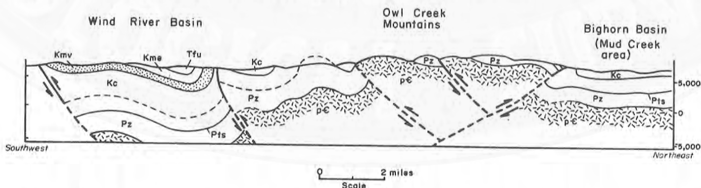
Figure 26. Structural cross section through the western Owl Creek Mountains from the Wind River Basin to the Bighorn Basin, Wyoming. Elevations are in feet above sea level. Cross section location is shown on Sheet 1 (back pocket) and Figure 3. (See Table 2 for formation abbreviations.)
