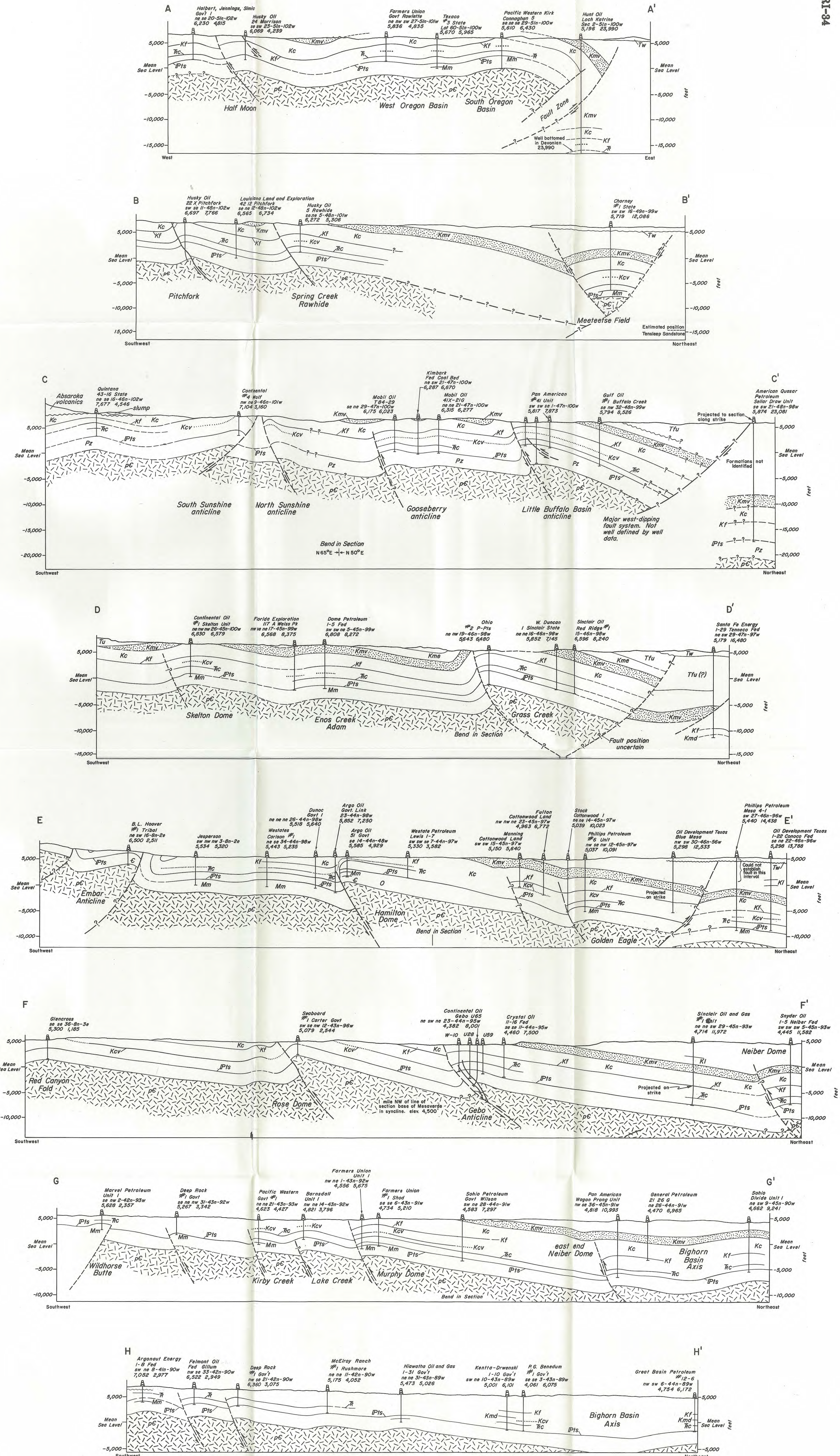
SHEET 2-REGIONAL STRUCTURAL CROSS SECTIONS, SOUTHERN BIGHORN BASIN (Locations on Sheet 1)
