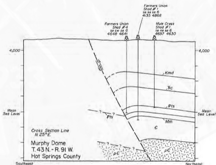
Figure 15. Structural cross section through the Murphy Dome, Big-horn Basin, Wyoming.
