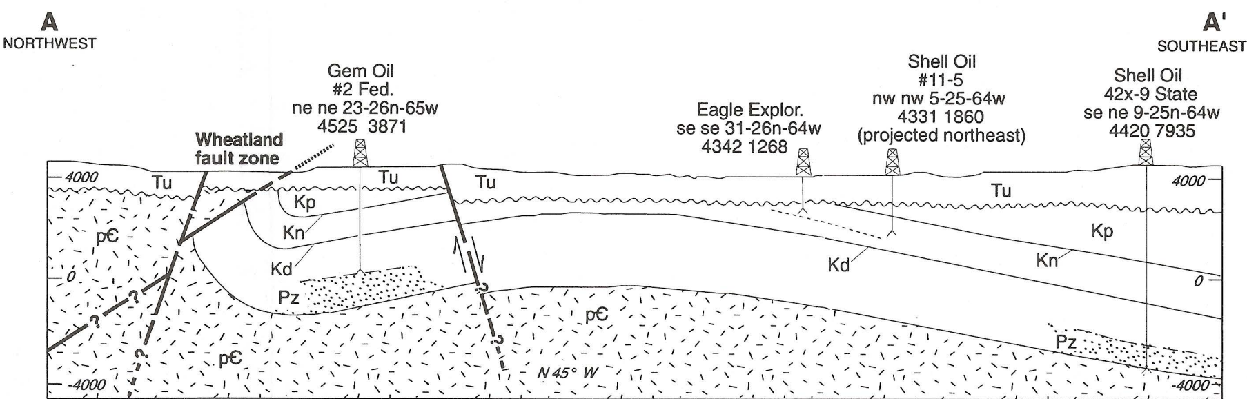
A. Northwest-southeast cross section A-A'.
