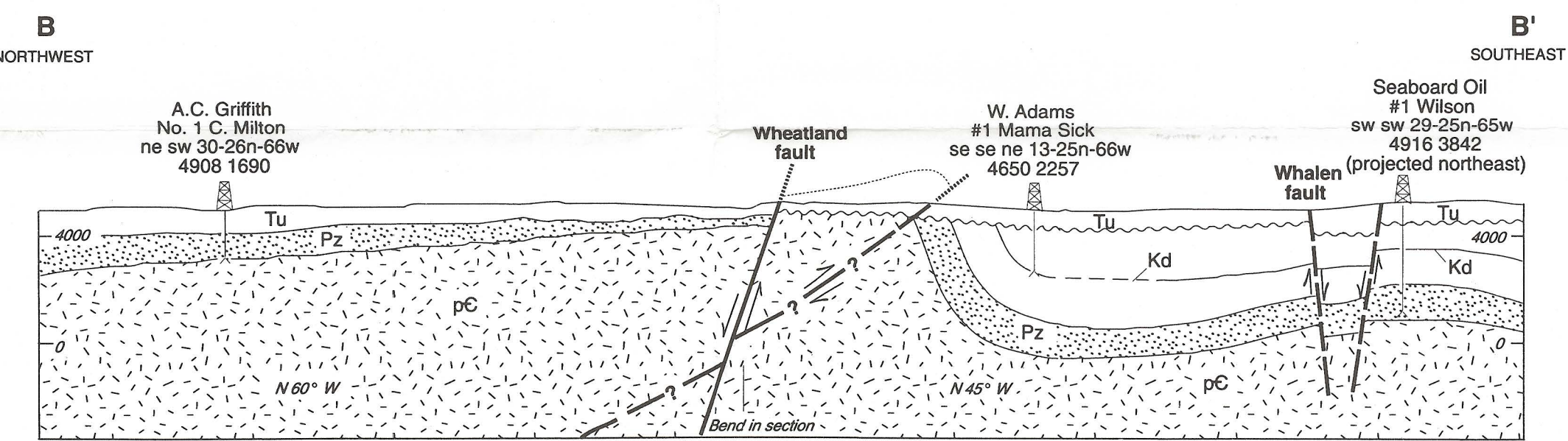
B. Northwest-southeast cross section B-B'.
