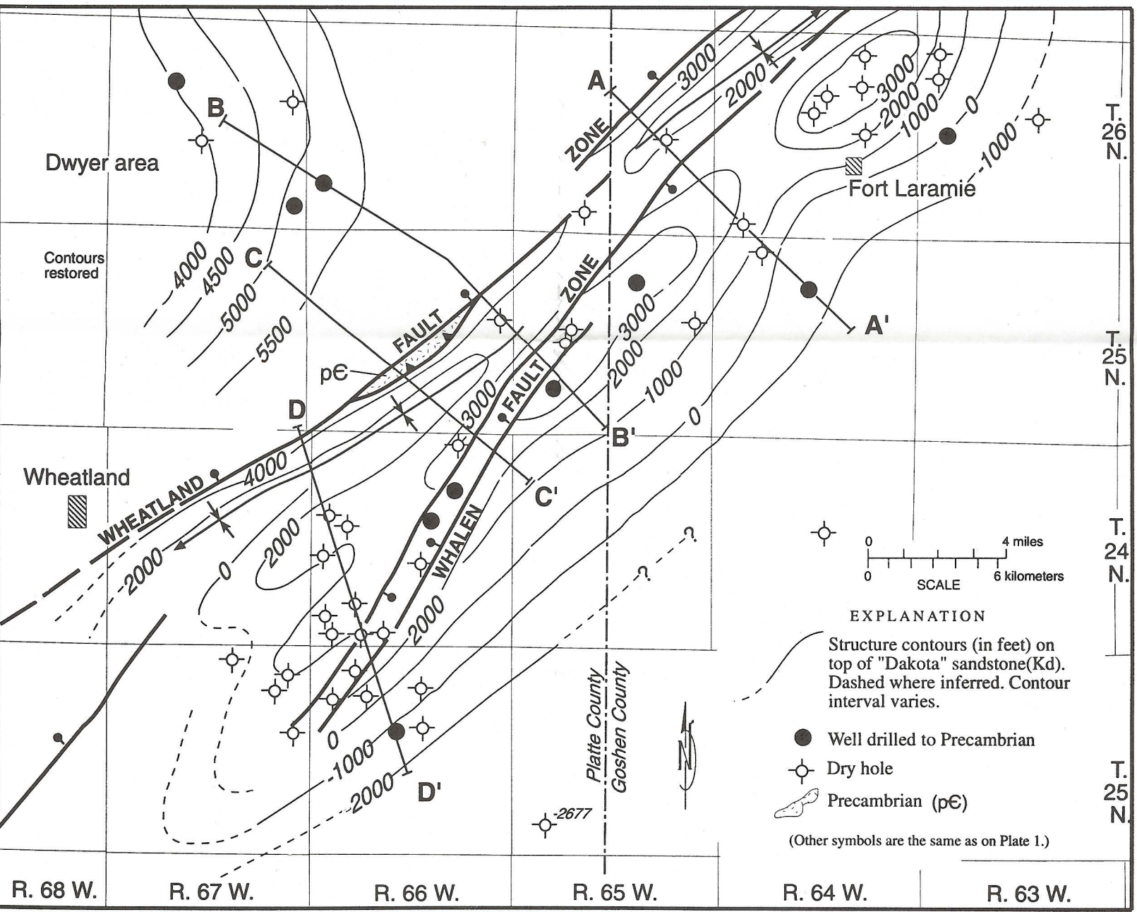
Detail Map 2. Structure contours on top of the "Dakota" sandstone (Cloverly Formation).
