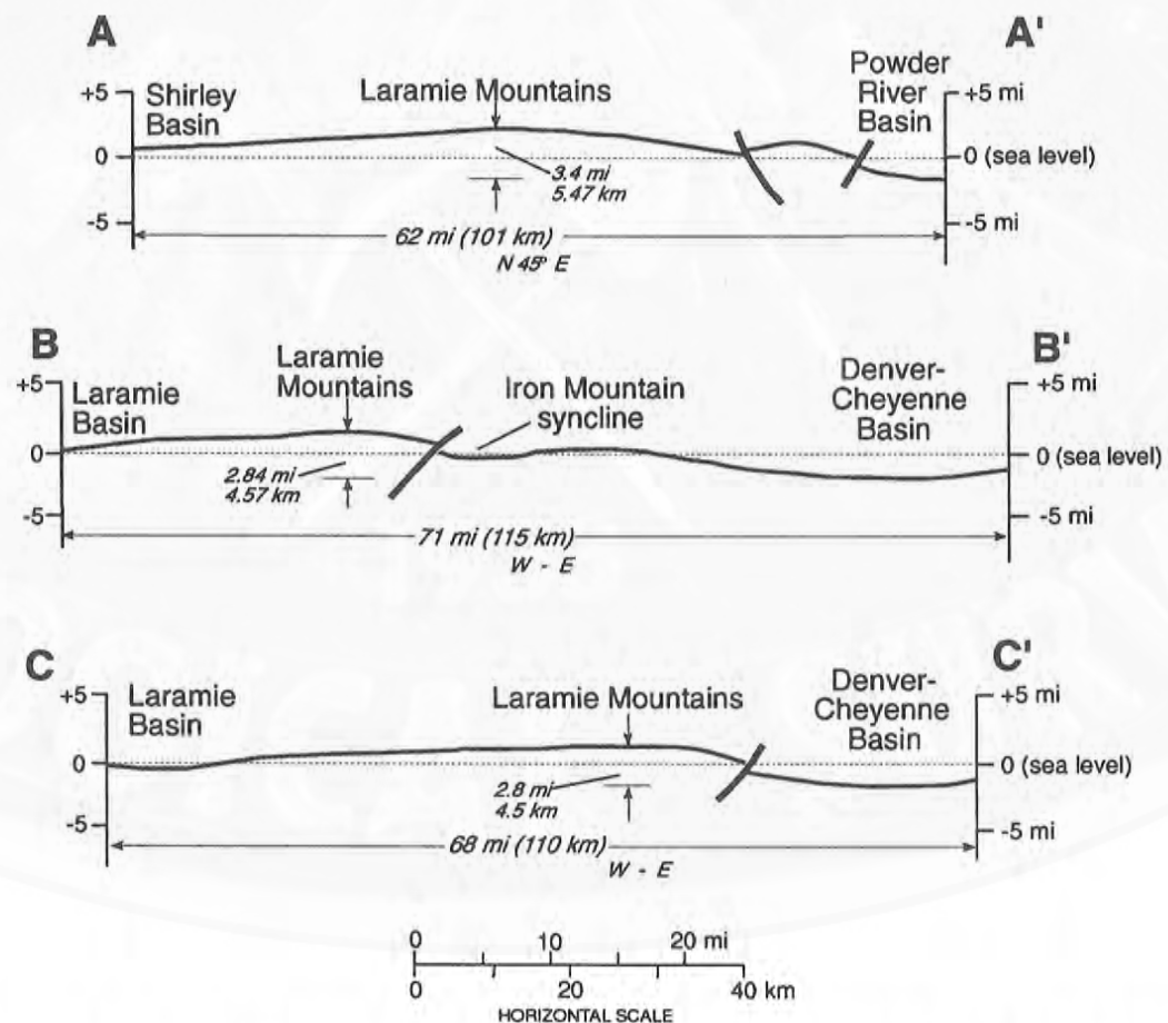
Figure 2. Foreland fold dimensions—wavelength and amplitude, southeastern Wyoming. Profile is at the top of the Precambrian basement or the Phanerozoic-Precambrian unconformity. Map shows approximate locations of cross sections A-A', B-B', and C-C'. Mi, miles; km, kilometers.
