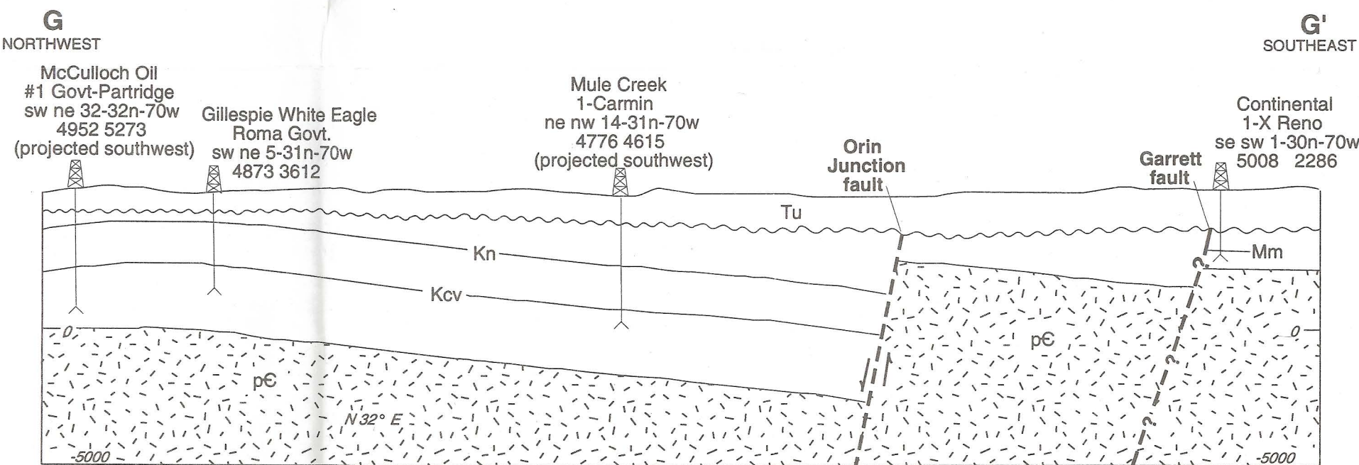
G. Northwest-southeast cross section G-G' across the Orin Junction and Garrett faults.
