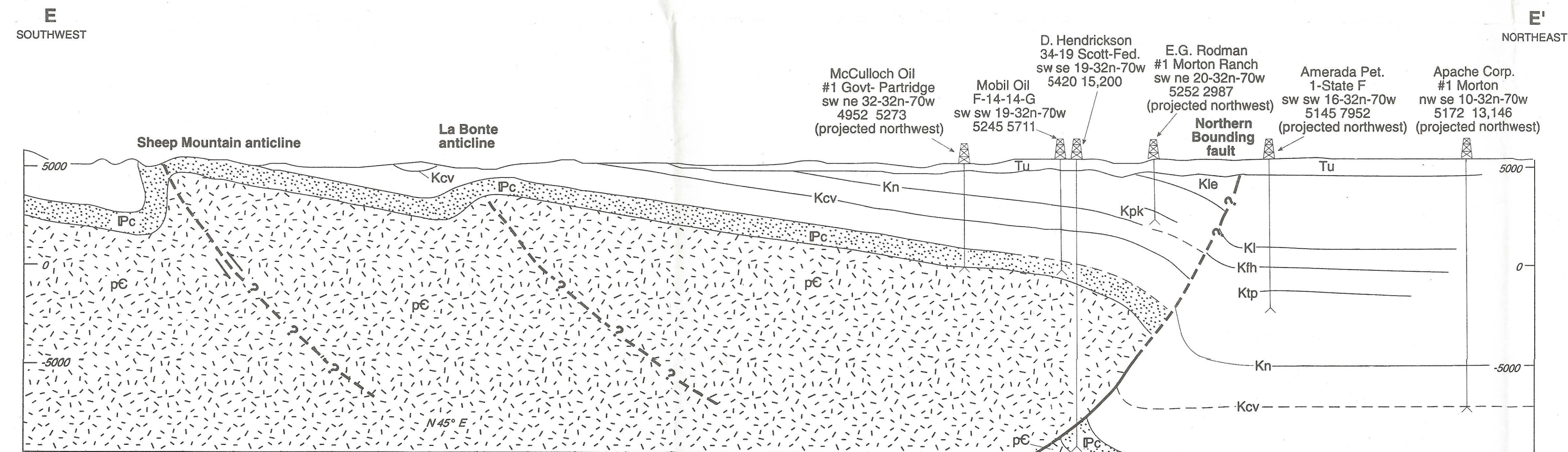
E. Southwest-northeast cross section E-E' across Sheep Mountain and La Bonte anticlines to the Northern Bounding Fault.
