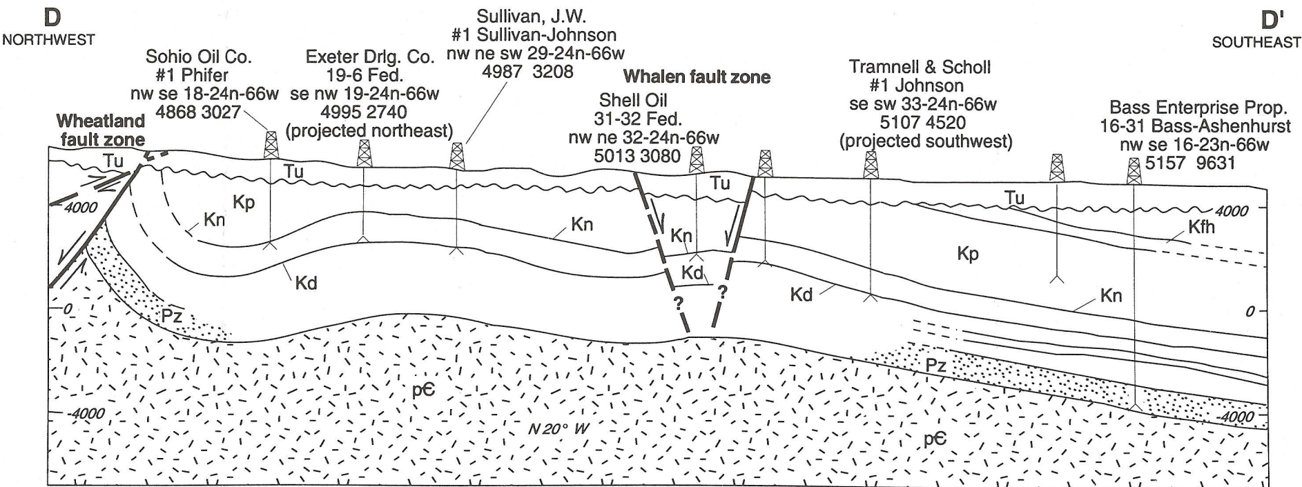
D. Northwest-southeast cross section D-D'.
