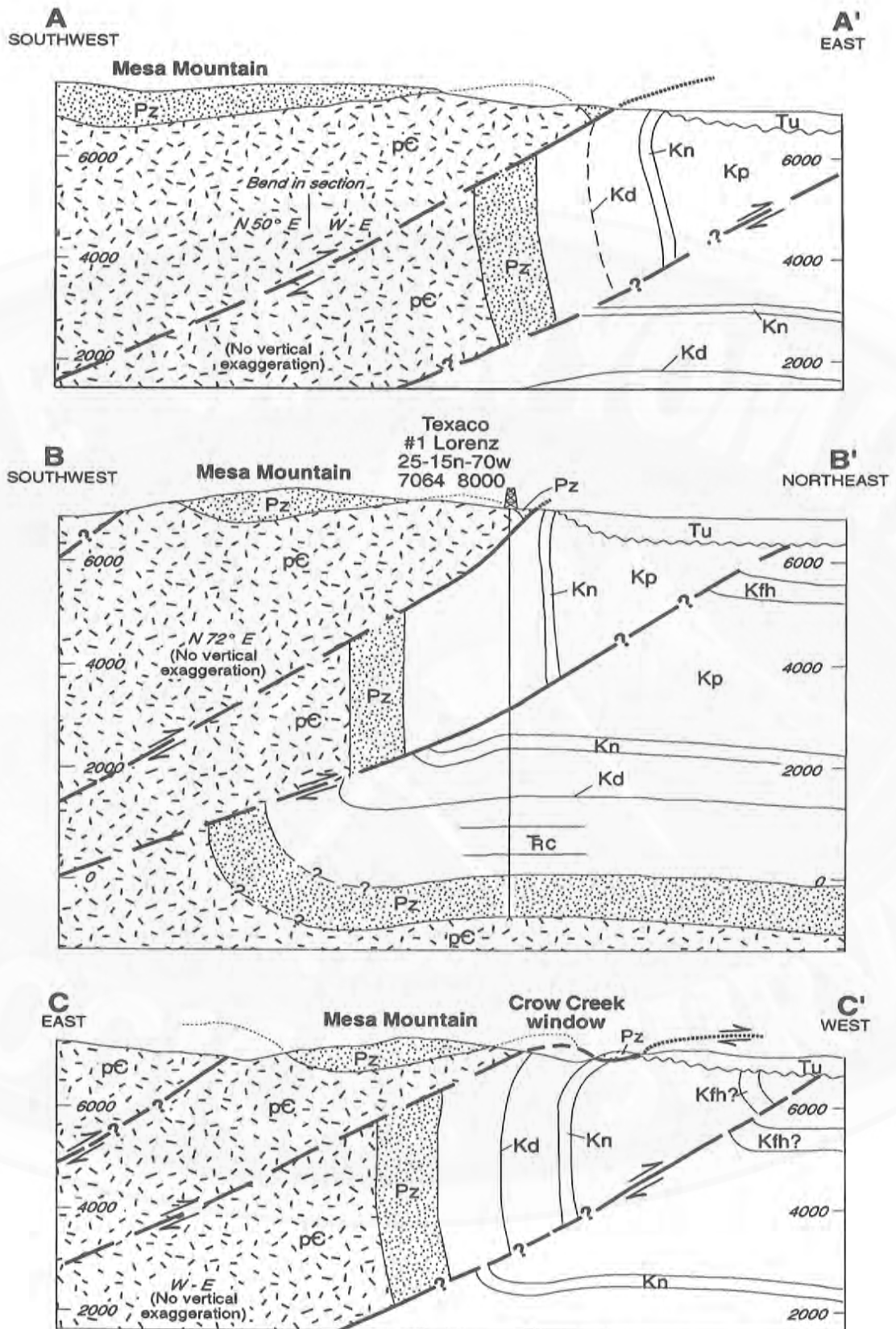
Figure 9. Cross sections A-A', B-B', and C-C' to accompany Detail Map 1 (Figure 8). Formation abbreviations are the same as on Figure 7, with the addition of: \overline{\text{Kc}} , Chugwater Formation; and Kd, "Dakota" sandstone (Cloverly Formation).
