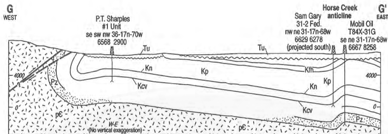
Figure 10. West to east cross section G-G' through Horse Creek siding to Horse Creek oil field. Location of cross section shown on Plate 1 . Formation abbreviations are: pC, Precambrian basement; Pz, Paleozoic rocks, undifferentiated; Kcv, Cloverly Formation; Kn, Niobrara Formation; Kp, Pierre Shale; Kfh, Fox Hills Sandstone; and Tu, Tertiary rocks, undifferentiated.
