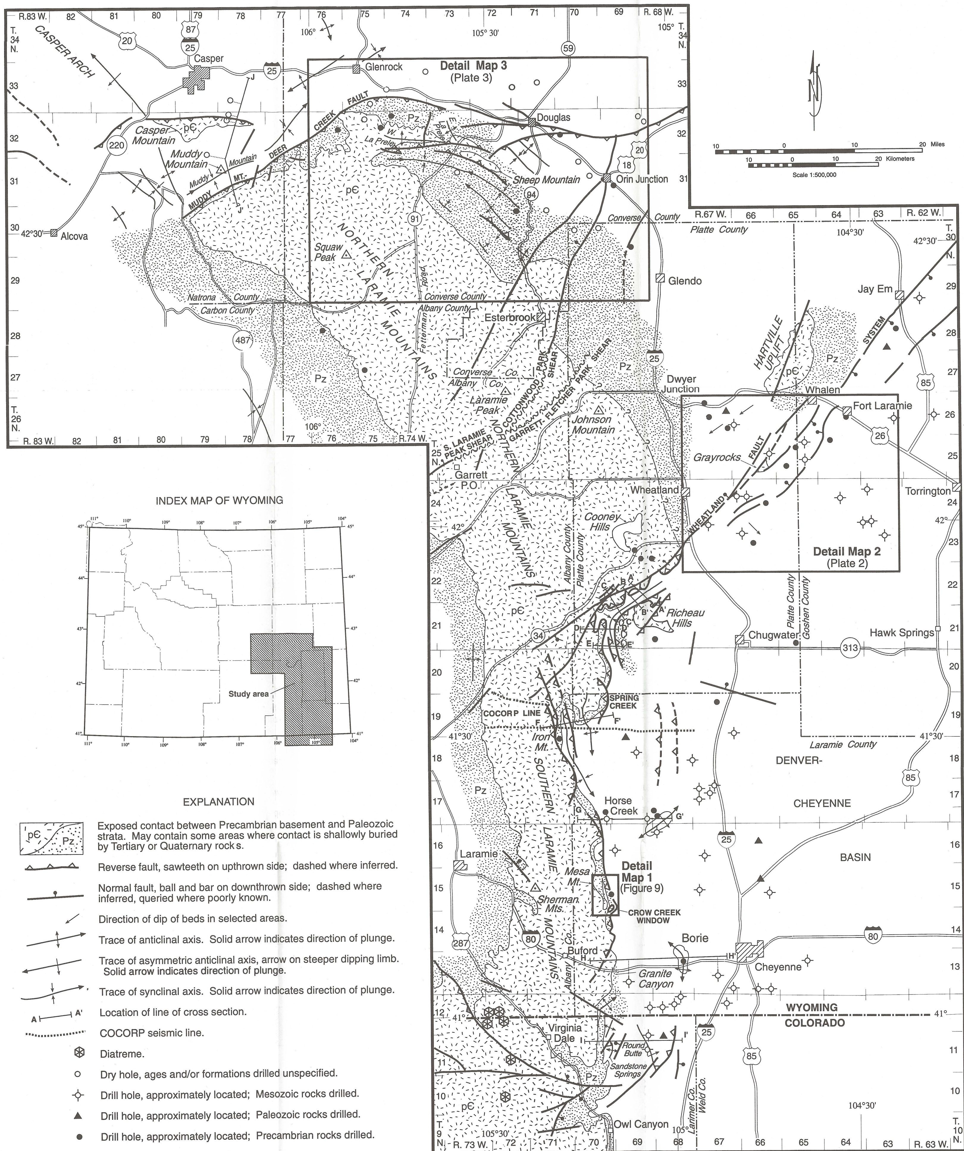
PLATE 1. GENERALIZED GEOLOGIC MAP OF THE SOUTHERN AND NORTHERN LARAMIE MOUNTAINS, NORTHERN COLORADO AND SOUTHEASTERN WYOMING, SHOWING LOCATIONS OF DETAILED MAPS, CROSS SECTIONS, AND SIGNIFICANT TEST WELLS.
