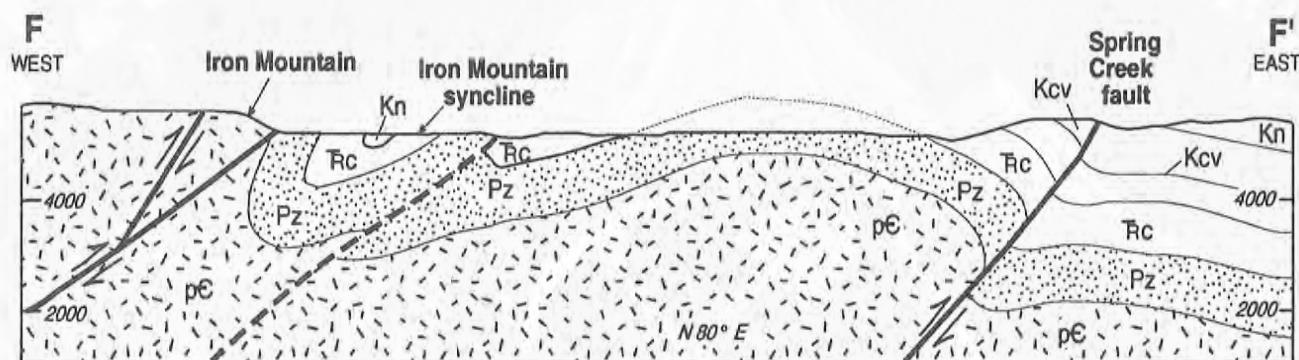
Figure 11. West to east cross section F-F' across Iron Mountain thrust fault, Iron Mountain syncline and anticline, and the Spring Creek fault. Location of cross section shown on Plate 1 . Formation abbreviations are the same as on Figure 10, with the addition of: Tc, Chugwater Formation.
