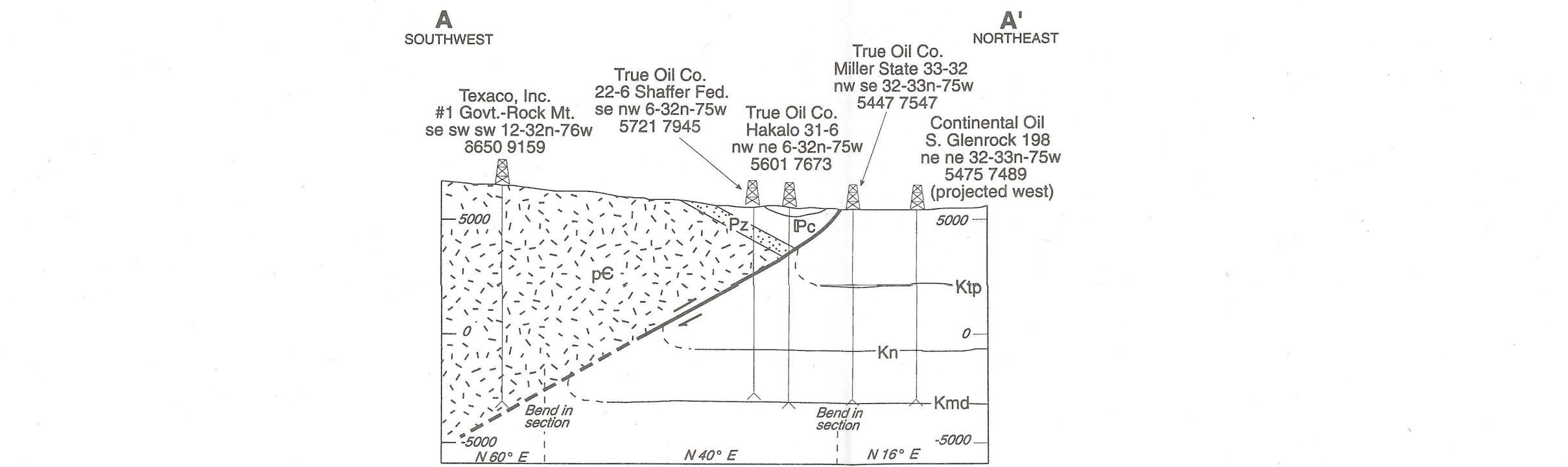
A. Southwest-northeast cross section A-A' across South Glenrock oil field.
