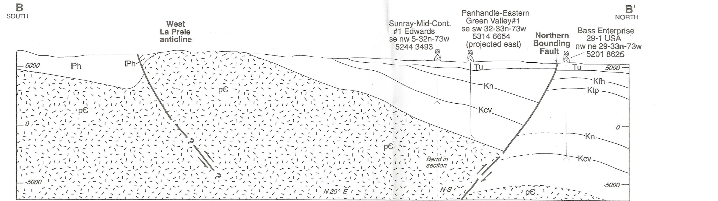
B. South-north cross section B-B' across West La Prele anticline.
