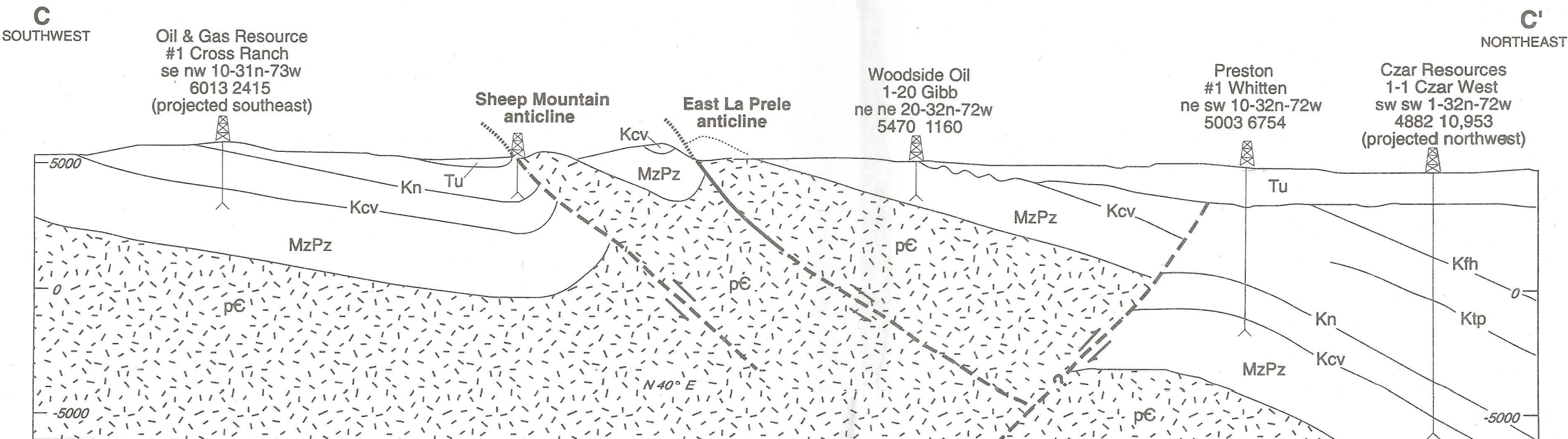
C. Southwest-northeast cross section C-C' across Sheep Mountain and East La Prele anticlines.
