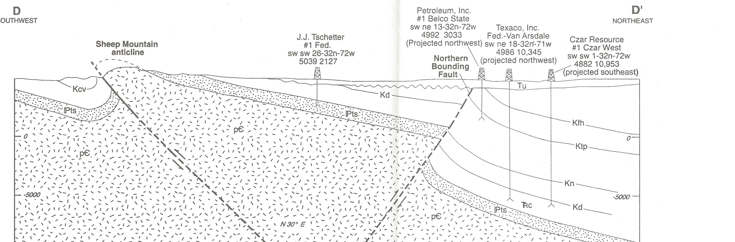
D. Southwest-northeast cross section D-D' across Sheep Mountain and the Northern Bounding Fault (NBF).
