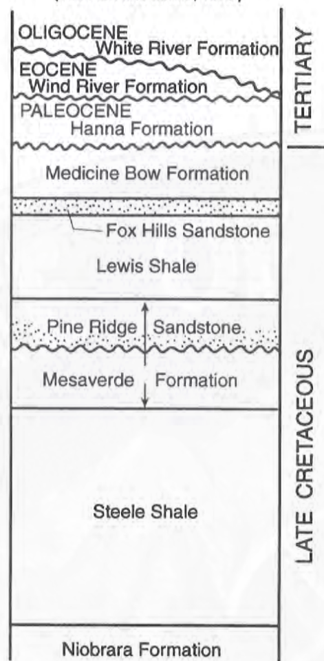
Figure 5. Stratigraphic sections of Late Cretaceous, early Tertiary, and Cenozoic deposits on the west and east sides of the southern Laramie Mountains. Undulating line represents an unconformity; stippled pattern indicates sandstone.
