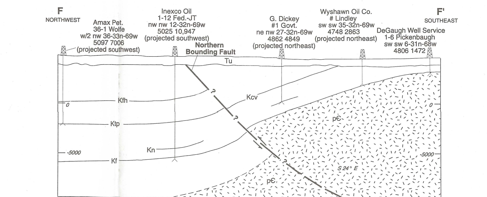
F. Northwest-southeast cross section F-F' across the Northern Bounding Fault in the vicinity of Shawnee, Wyoming.
