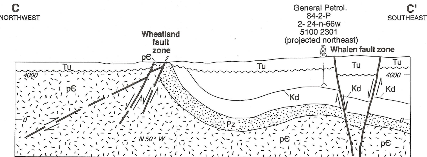
C. Northwest-southeast cross section C-C'.
