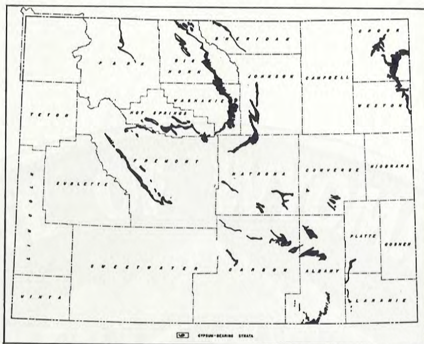
Fig. 3. Outcrop map of gypsum bearing strata.
