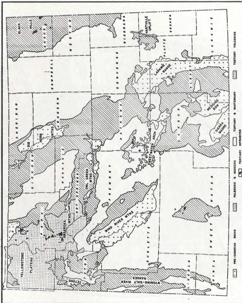
Fig. 1. Geologic index map of Wyoming.
