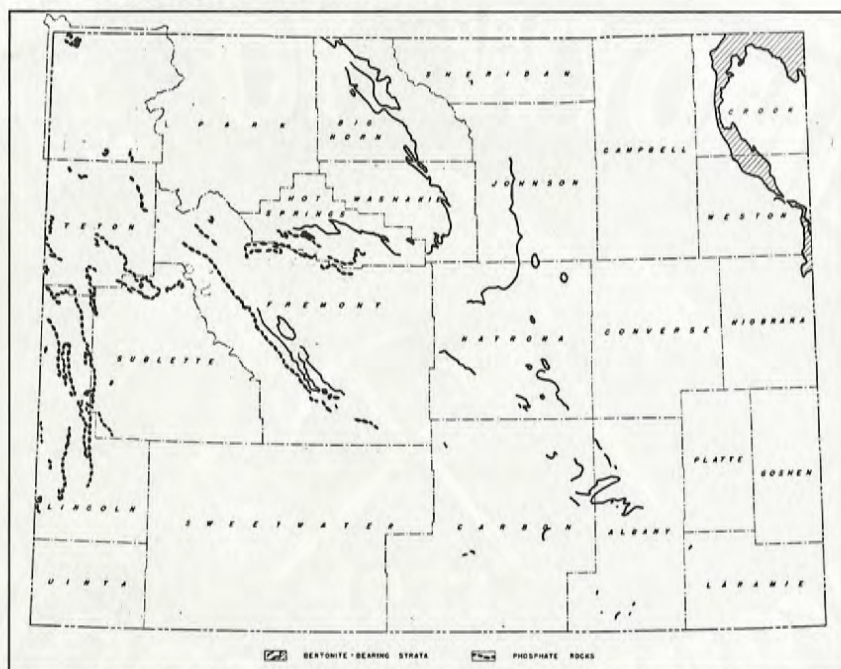
Fig. 2. Outcrop map of bentonite and phosphate bearing strata.
