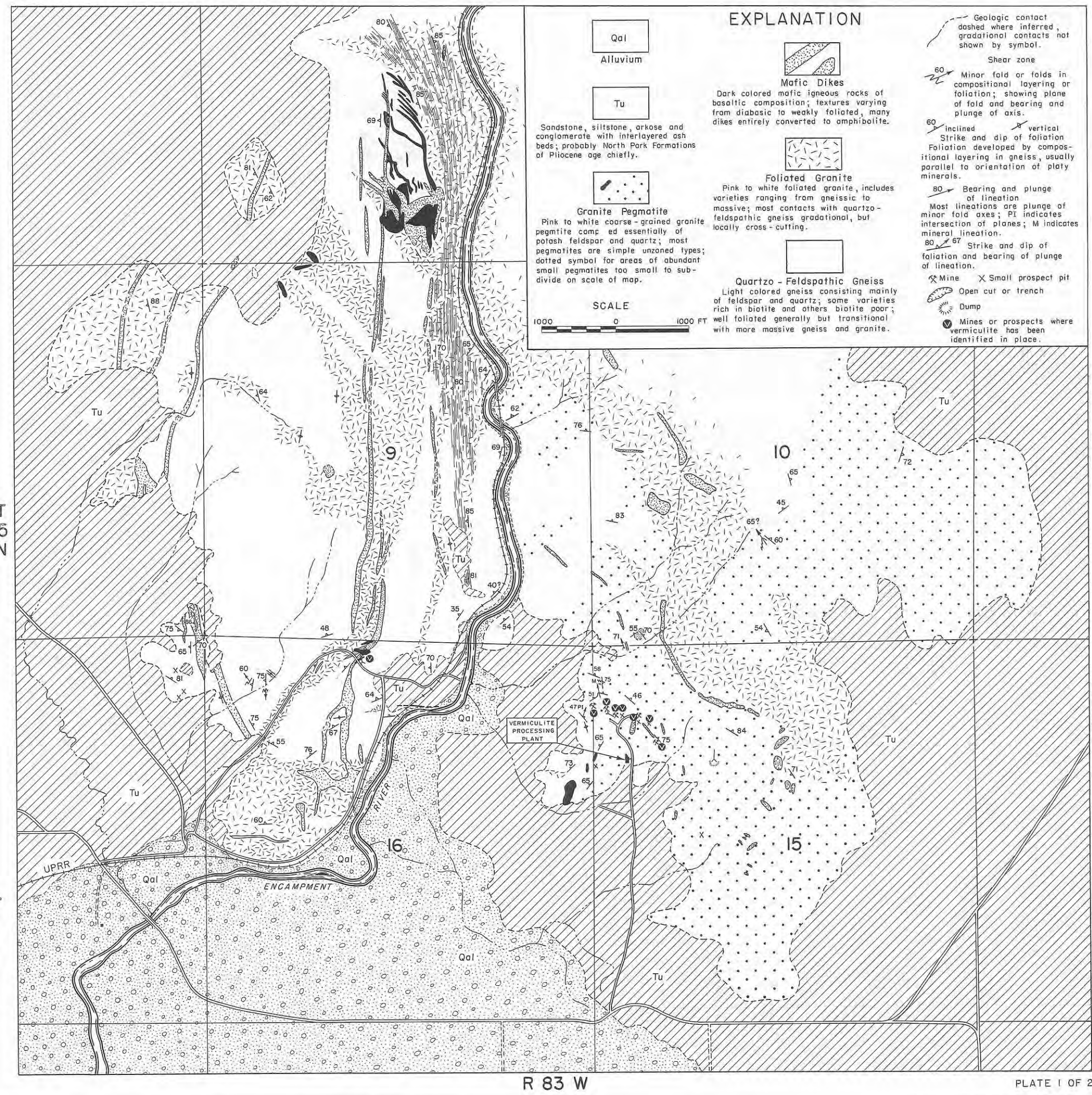
Geologic Map showing vermiculite deposits of the Baggot Rocks area, Carbon County, Wyoming
