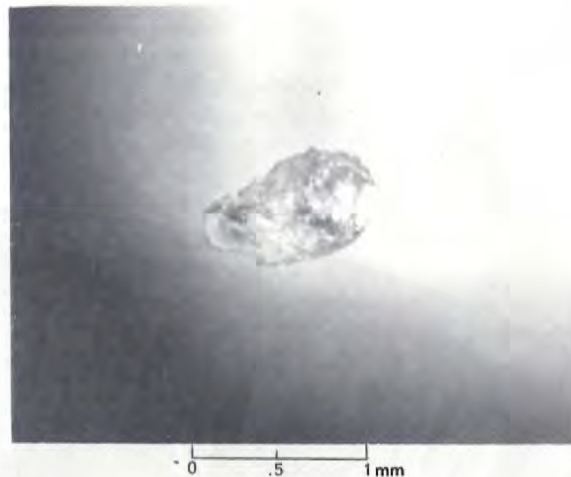
Figure 22 — Aggregate diamonds from State-Line kimberlite pipes. A) Aggregate crystal (SD1-X1) from the Sloan 1 pipe showing complex intergrowth of octahedra. B) Rounded aggregate crystal (SD1-X1) of intergrown octahedra and dodecahedra from the Aultman pipe, Wyoming. C) SEM micrograph of interpenetrant twin of planar octahedra from the Sloan 2 pipe. (First diamond recovered from Colorado kimberlite).
