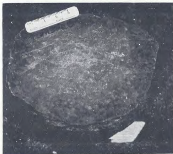
Figure 17 — Slabbed surface of serpentinized diamond-bearing garnet peridotite nodule showing dominantly tabular texture with narrow zones of porphyroclastic to mosaic texture. A) Entire nodule. B) Enlarged portion of surface.
