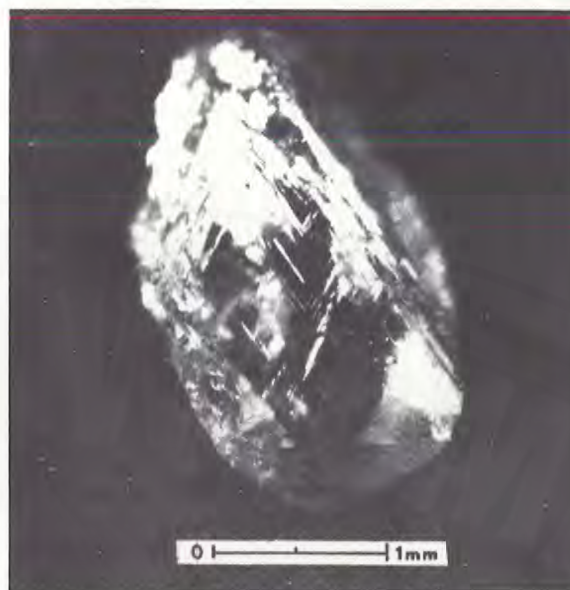
Figure 18 — Distorted octahedral diamond from the Sloan 2 kimberlite pipe. It is the largest diamond recovered to date from the State-Line district.
