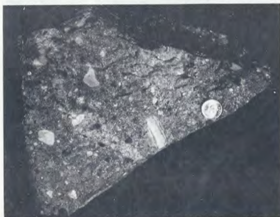
Figure 7 — Kimberlite samples. A) Kimberlite breccia, light colored fragments are mostly sedimentary carbonates and igneous carbonatites. B) Angular block and several small rounded fragments (gray) of Lower Paleozoic limestone in kimberlite
