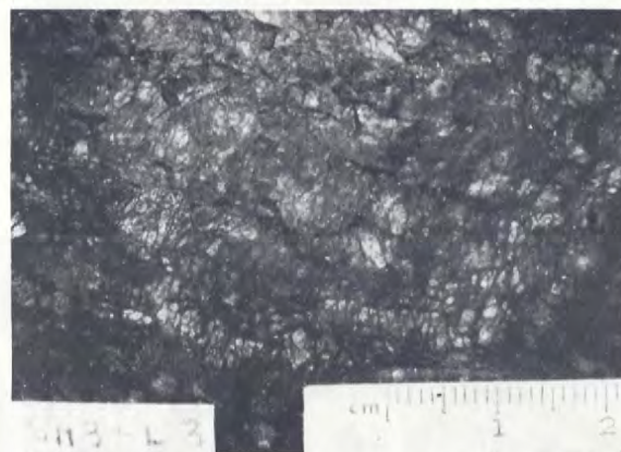
Figure 17 — Slabbed surface of serpentinized diamond-bearing garnet peridotite nodule showing dominantly tabular texture with narrow zones of porphyroclastic to mosaic texture. A) Entire nodule. B) Enlarged portion of surface.
