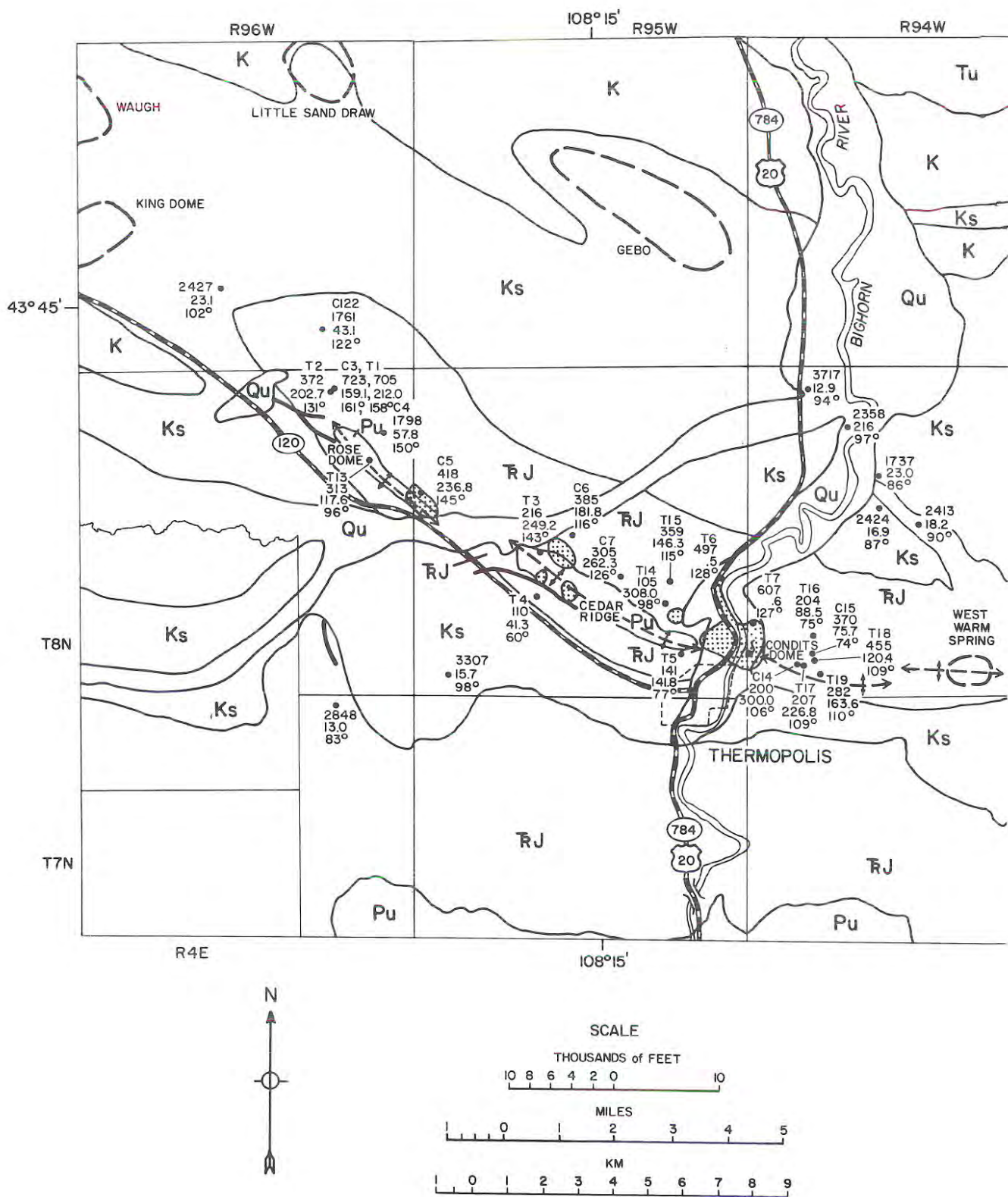
Figure 4. Geologic and thermal data for the Thermopoles Anticline area.
