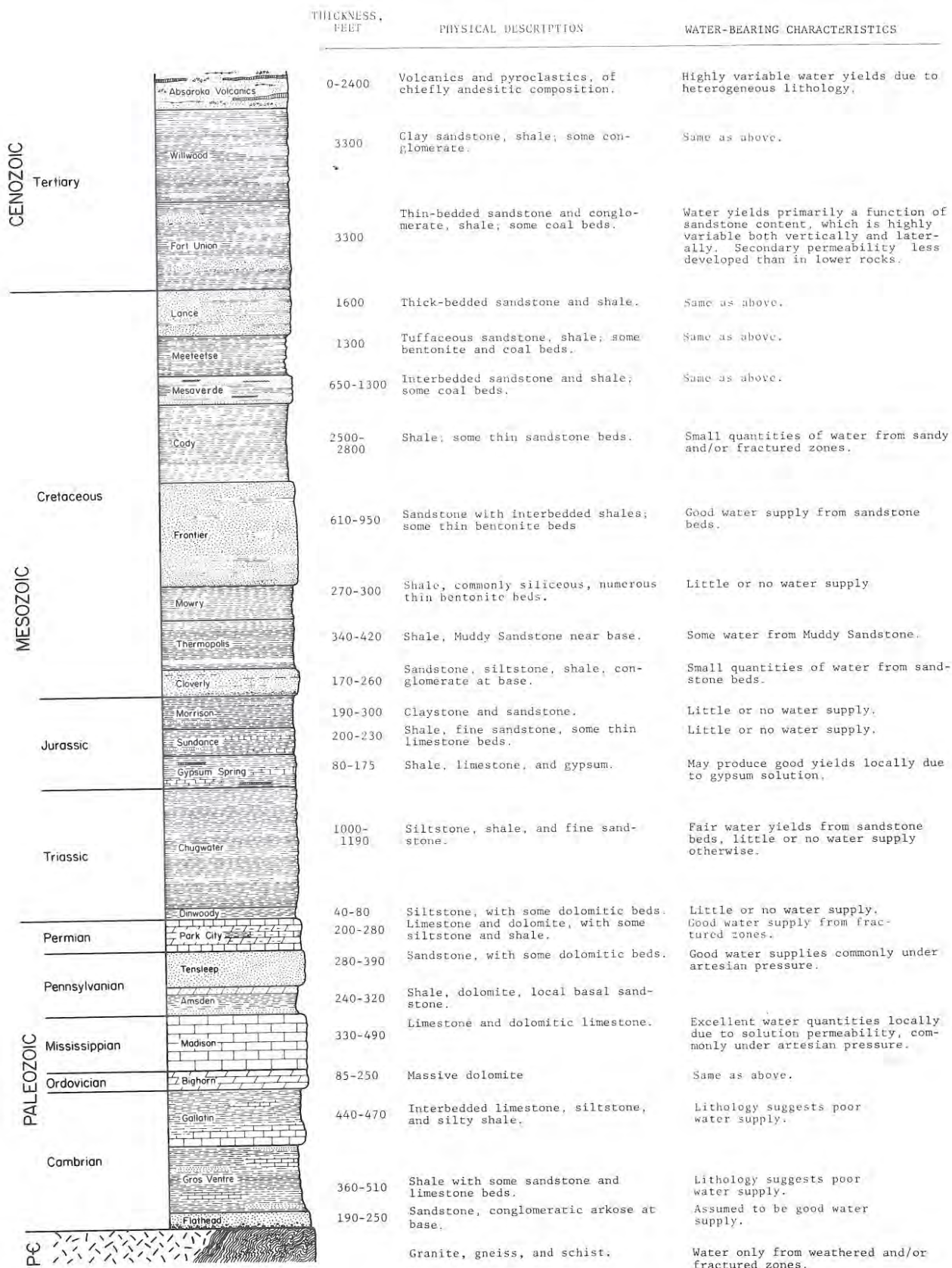
Figure 3. Geologic column for the Thermopolis study area. See page 43 for credits. Column thicknesses are to scale 1:12,000 for Frontier and below, 1:52,800 for Cody and above.
