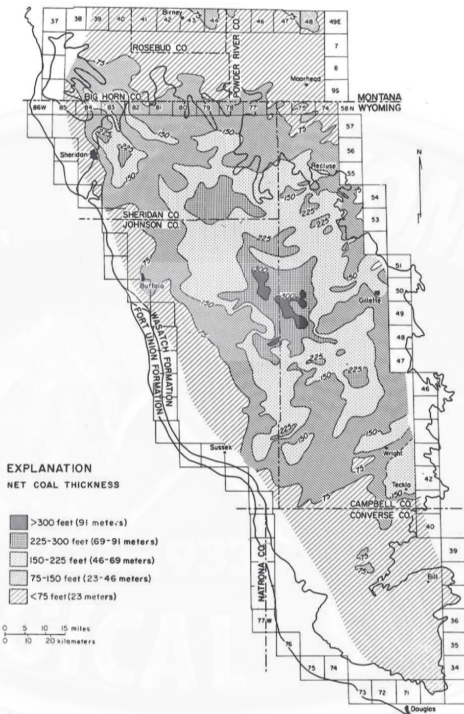
Figure 10. Coal isolith map showing that the net thickness of coal is greatest in the center of the Wyoming part of the basin and northeast of Sheridan, Wyoming. Net thickness is nearly zero between Buffalo and Sussex, and between Douglas and Bill, Wyoming, which were areas of muddy lacustrine sedimentation.
