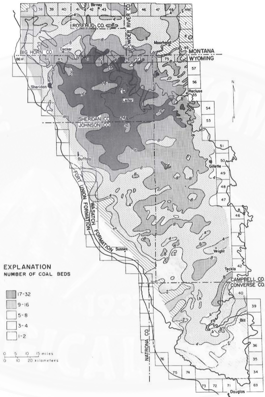
Figure 11. Coal isopleth map revealing that the greatest number of coal seams is in the north-central part of the basin. In the two areas of thick strike-parallel coals (Figure 9) there are fewer seams, but they have a greater average thickness (Figure 12). Few seams are present along the west and south margins of the basin.
