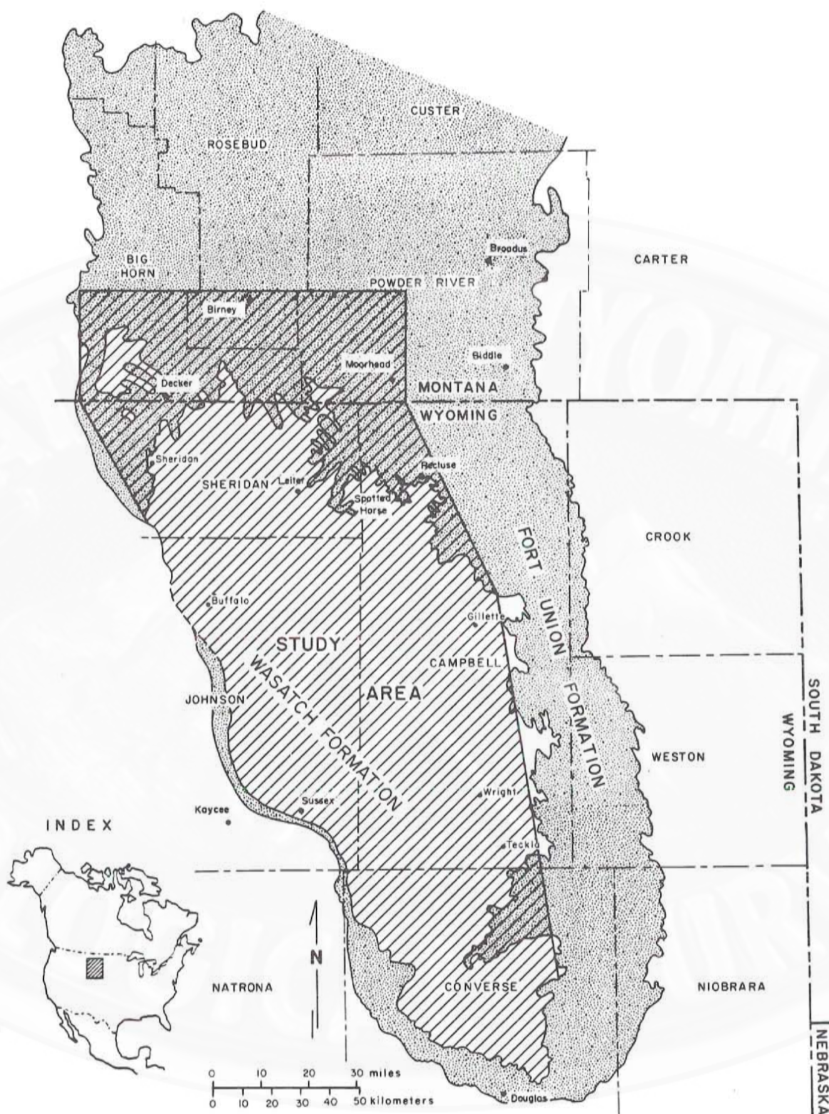
Figure 1. Location of the study area in the Powder River Basin. Geologic contacts are from Love and others (1955) and Ross and others (1955). The structural asymmetry of the basin is apparent from variations in the width of outcrops. Note that much of the Wyoming part of the study area is overlain by the Wasatch Formation.
