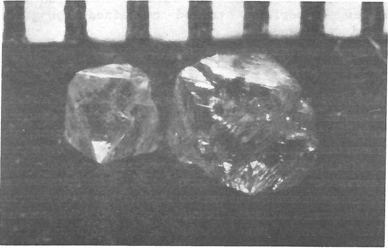
Figure 5. Some Wyoming diamonds -- note the typical octahedral shape (scale division 1 mm apart).
