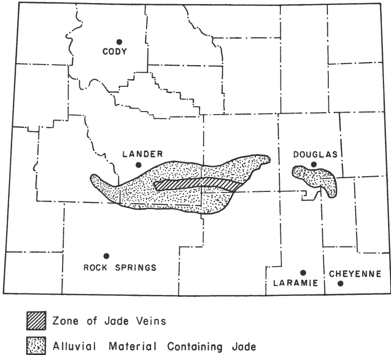
Figure 7. Principal jade occurrences of Wyoming.
