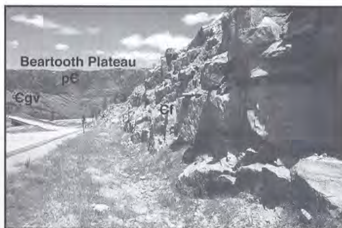
Figure 32. Outcrop of Flathead Sandstone (Cf) north of bridge over Sunlight Creek. The Flathead is about 100 feet of well-cemented brown quartzitic sandstone. Gros Ventre Shale (Egv) in slopes behind bridge, Precambrian (pC) on Beartooth Plateau in distance. (Photograph by D.D., 1996.)
