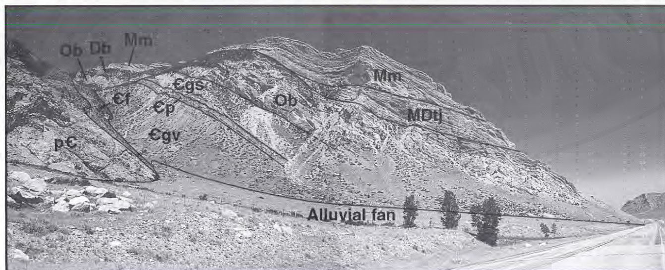
Figure 20. Panorama of the lower Paleozoic section exposed along the north side of Clarks Fork Canyon near the canyon mouth. Formation symbols are: pC, Precambrian; Cf, Flathead; Egsv, Gros Ventre; Ep, Pilgrim Limestone; Egs, Grove Creek and Snowy Range; Ob, Bighorn; MDtj, Three Forks and Jefferson; Db, Beartooth Butte; and Mm, Madison. (Photographs by H.P.H. and A.D., 1996.)
