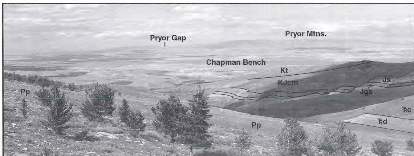
Figure 25. View to northeast across northern part of Bighorn Basin. Chapman Bench in middle distance, Pryor Mountains and Pryor Gap on skyline. Formation symbols are: Pp, Phosphoria; Fd, Dinwoody; Fc, Chugwater; Jgs, Gypsum Spring; Js, Sundance; KJcm, Morrison and Cloverly; and Kt, Thermopolis. (Photograph by D.D., July, 1996.)
