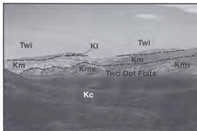
Figure 22. View to east of Cody Shale (Kc in foreground), Mesaverde (Kmv, tree-covered ridge), Meeteetse (Km, brown and gray banded rocks), Lance (Kl, brown, tree-covered ridge on left skyline), and Willwood (Twi, red and white banded rocks on right skyline) Formations. Willwood Formation unconformably overlies the Meeteetse and Lance Formations here and the Cody and Mesaverde to the north. (Photograph by H.P.H., July, 1996)
