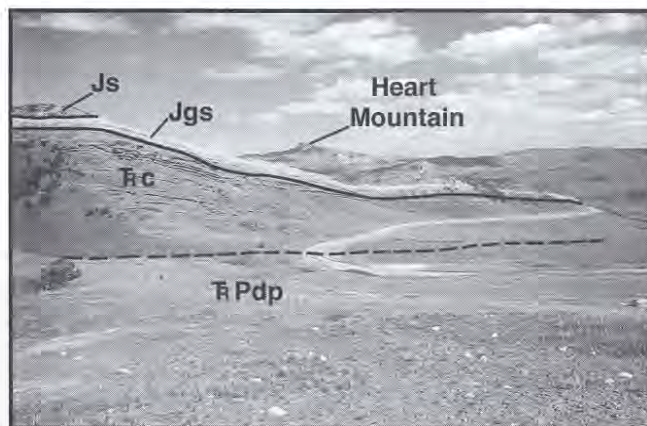
Figure 24. View to southeast from dip slope on Phosphoria/Dinwoody (Pdp). The red Chugwater (C) is 650-750 feet thick and is overlain by the white Gypsum Spring (Gs, the white gypsum bed at the base of the formation is up to 50 feet thick) and the Sundance (Js, at the top of the exposure). Heart Mountain on the skyline in center of photograph. (Photograph by D.D., July, 1996.)
