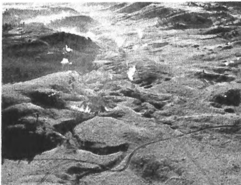
Figure 3. November 1975, eastward aerial oblique view of surface effects of an underground mine fire above the northern part of the Acme mine, Wyoming (from Dunrud and Osterwald, 1980).
