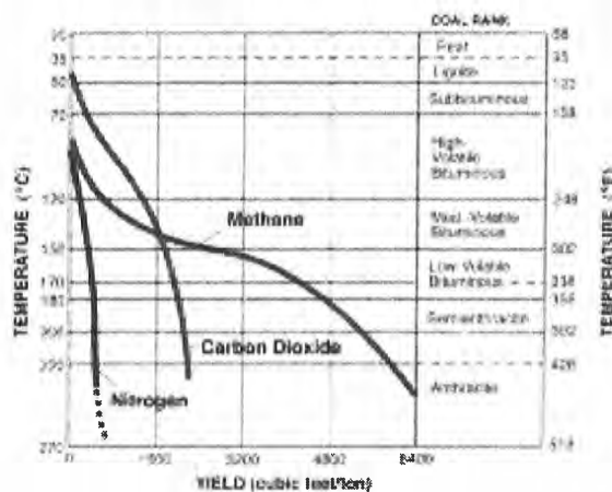
Figure 6. Calculated curves of gases generated by thermogenesis from coal during coalification (from De Bruin and others, 2000 as modified from Rightmire, 1984).
