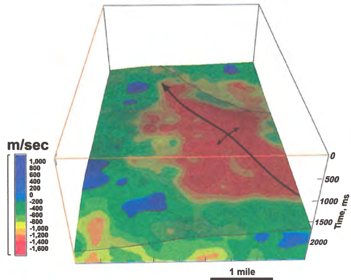
Figure 20. Anomalous velocity model of the Mowry Shale generated from a 3-D seismic survey in the Greater Green River Basin, Wyoming. A significant anomalously slow velocity domain, occurring at the top of the Mowry Shale and associated with an anticline, is clearly defined.
