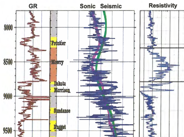
Figure 2. Typical well log of the Mowry Shale characterized by high gamma ray counts, lower interval velocities, and higher resistivities.
